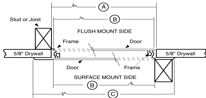
SECTION DETAIL
