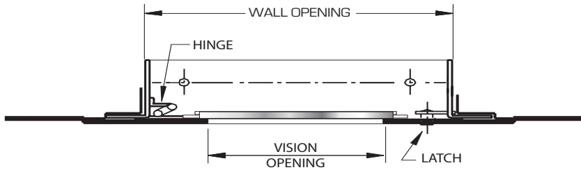
SECTION DETAIL
