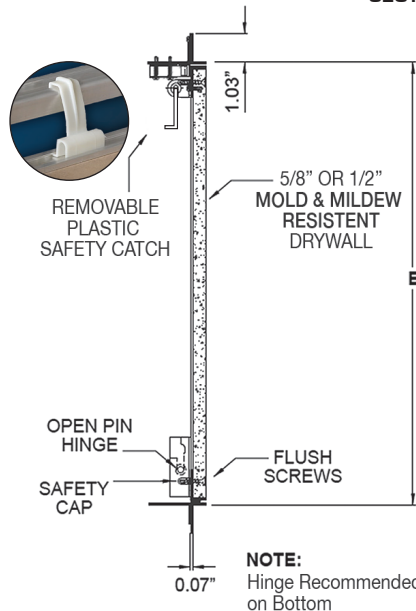
Heavy duty reinforced plastic corners ensures flush installation
