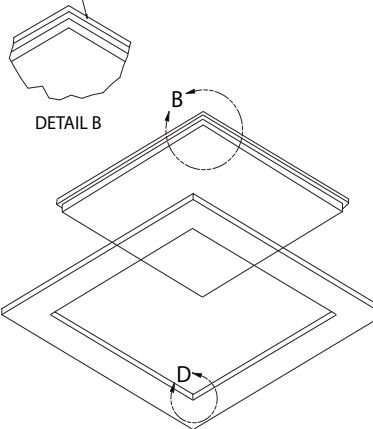
SEALED DRYWALL EDGES CORNER DETAIL
